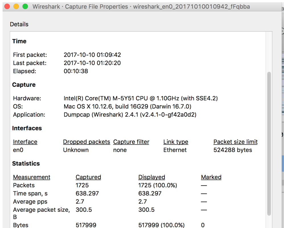
Figure 1.10 Capture File Properties window
